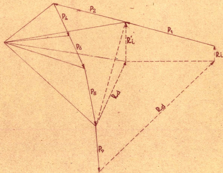
POLIGONO VECTORIAL
